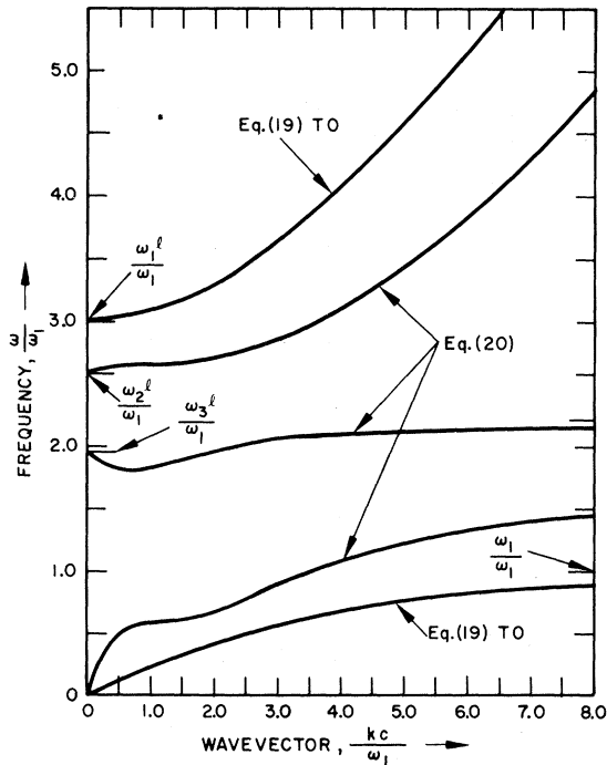
FIG. 5. \omega versus k for small- k values for \vec{k} in the x_2x_3 plane. Orthorhombic case II. Parameter values same as for Fig. 3. \epsilon_1^\infty = 2 , \epsilon_2^\infty = 3 , \epsilon_3^\infty = 4 , \epsilon_1^0 = 18 , \epsilon_2^0 = 12 , \epsilon_3^0 = 6 , \omega_2 = 1.3\omega_1 , \omega_3 = 1.6\omega_1 . The branches do not cross because of the particular parameter values chosen. \phi_2 = \phi_3 .
