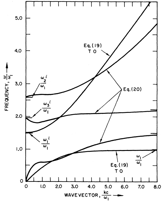
FIG. 6. Same as Fig. 5 except that \epsilon_1^\infty and \epsilon_1^0 were changed in order to illustrate that the two transverse branches do cross the other three branches \epsilon_1^\infty = 2 , \epsilon_1^0 = 4.5 . The crossing occurs because (19) is independent of (20).
