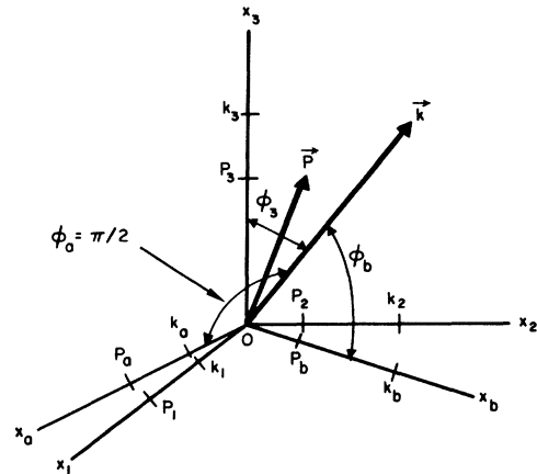
FIG. 9. Special polarization component directions with respect to a general \vec{k} vector. Uniaxial case IV.
